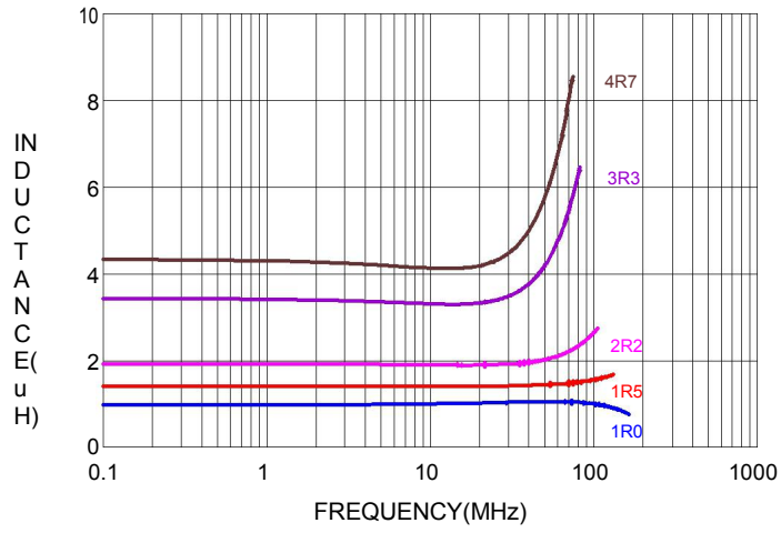
SMDH2012B-SERIES
