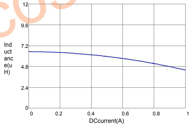
SMDH3010TF-6R8
