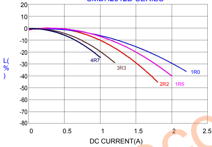
SMDH2012B-SERIES
